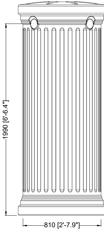
Hinteransicht / View from back Vista de atrás / Vue arrière
